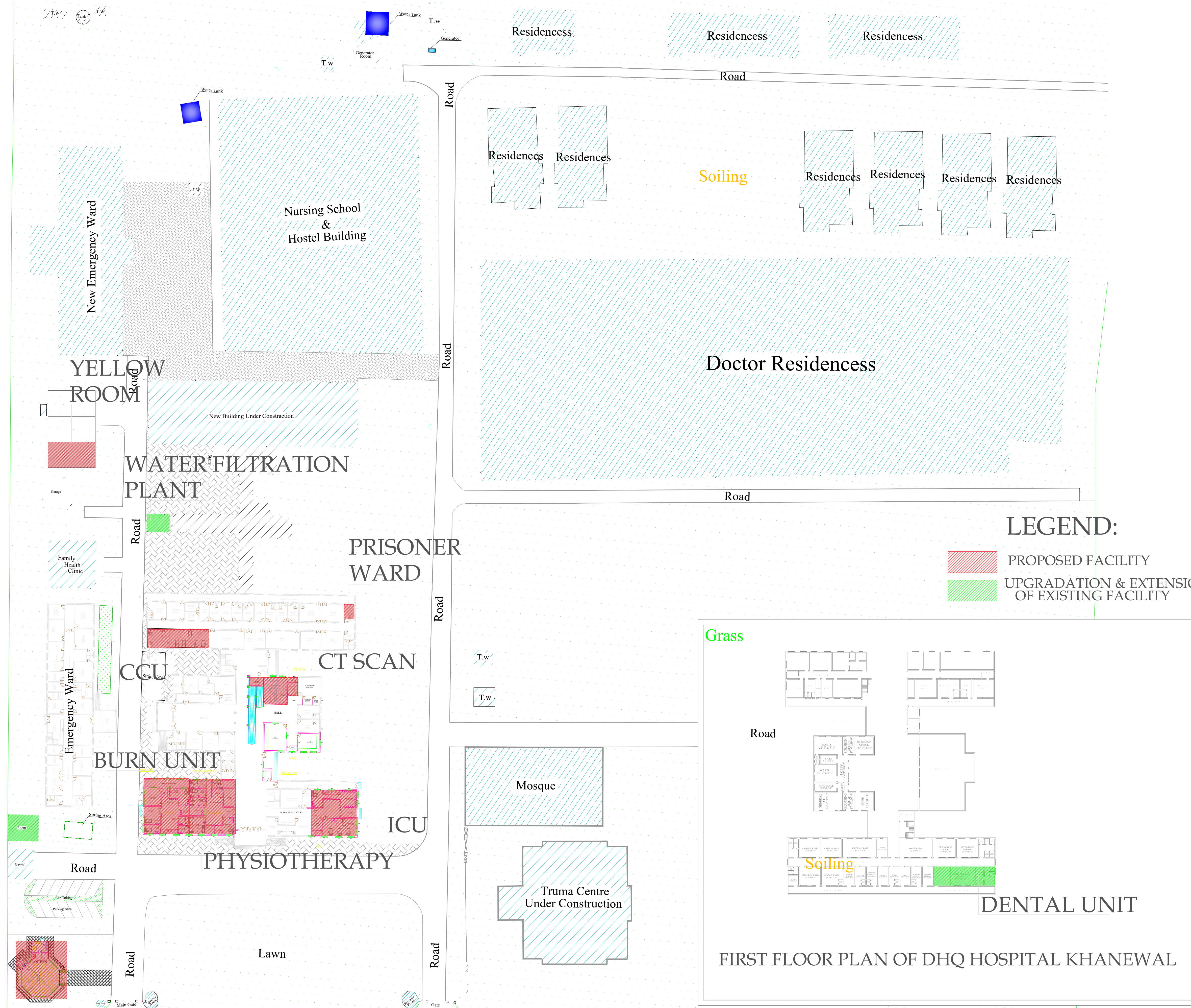
MASTER PLAN OF DHQ HOSPITAL KHANEWAL
